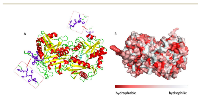
Fig. 2 A: Visualization of the secondary structure of N-terminal Histagged (R)-selective \omega -transaminase from Arthrobacter sp. (His 6 -ATA-117). In purple the histidine tag and in cyan the PLP cofactor, enzyme diameter: 7.17 nm. B: Surface hydrophobicity: in red the hydrophobic areas and in light-grey the hydrophilic areas. The enzyme structure was predicted using AlphaFold software, figures and the enzyme diameter was obtained using PyMOL software.
