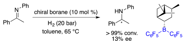
Scheme 2 Initial asymmetric hydrogenation catalyzed by a chiral borane.
