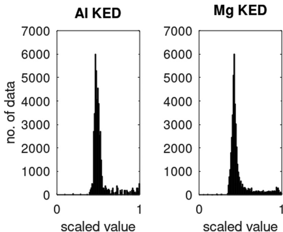
Fig. 1 Distributions of kinetic energy densities \tau_k of crystalline aluminium and magnesium computed as described in ref. 19. The values are scaled to [0, 1].
