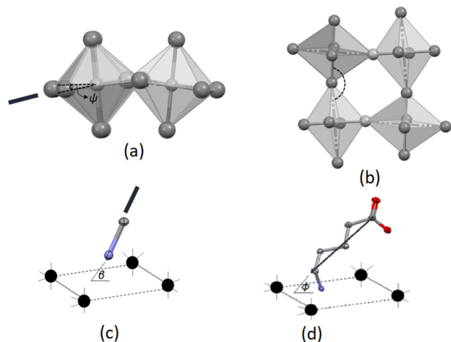
Fig. 2 Illustration of structural descriptors: (a) \psi angle (b) Mn–Cl–Mn bridging angle indicated by black dashed lines (c) \beta angle and (d) \phi angle.
