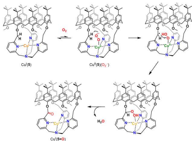
Fig. 6 Proposed mechanism for intramolecular C–H bond oxidation upon O_2 activation in Cu(I) ( 5 ). A similar pathway is proposed for Cu(4) .
