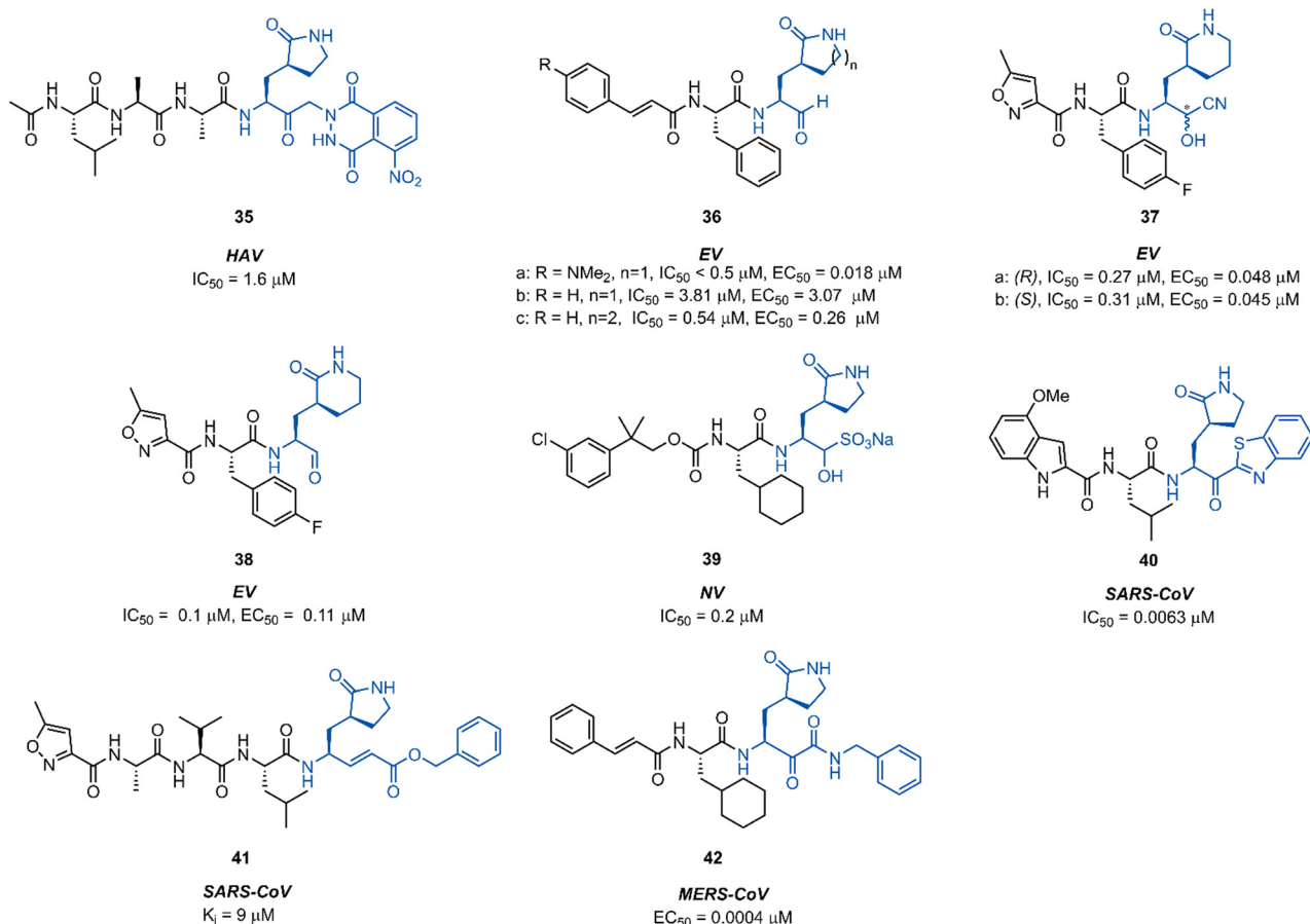
Fig. 10 Representative examples of inhibitors targeting 3C/3CL pro containing a P 1 (S)- \gamma/\delta -lactam isostere.
