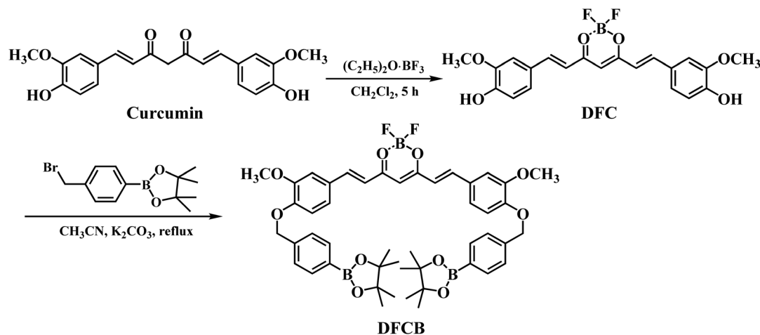
Scheme 1 The synthesis route for the DFCB sensor.
