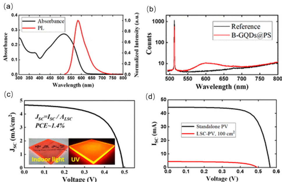
Fig. 13 (a) Absorbance and PL spectra of C-dots embedded in the PS solid matrix. (b) Experimental raw data of an absolute QY measurement. (c) The J-V curves for LSCs (100 cm 2 ). (d) The J-V curves for standalone PVs and LSCs-PVs. Reproduced with permission from ref. 175. Copyright 2022, American Chemical Society.
