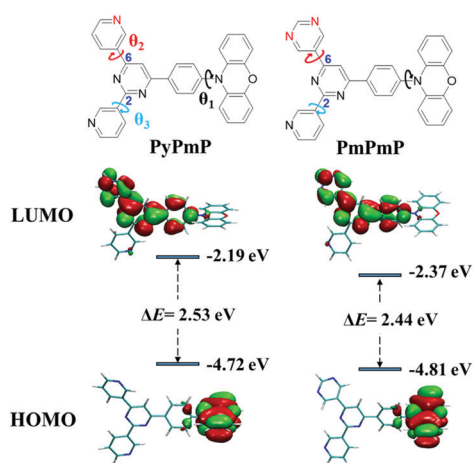
Fig. 1 Molecular structures of PyPmP and PmPmP and their simulated HOMO/LUMO energy levels and spatial distributions. The isovalue is 0.02.
