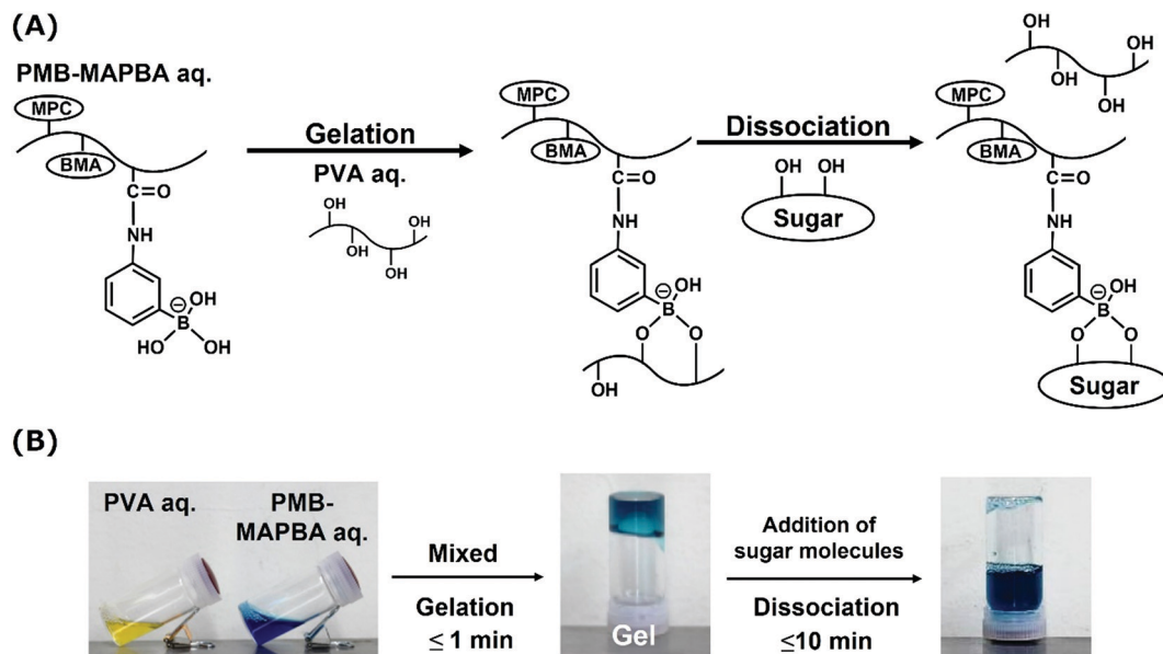
Fig. 4 (A) A schematic illustration of the gelation and dissociation mechanisms of the PMB-MAPBA/PVA hydrogel. (B) Photographs of PMB-MAPBA and PVA aqueous media (labeled with dye) and the PMB-MAPBA/PVA hydrogel. The addition of sugar molecules immediately induced the dissociation of the hydrogel (in 10 min).
