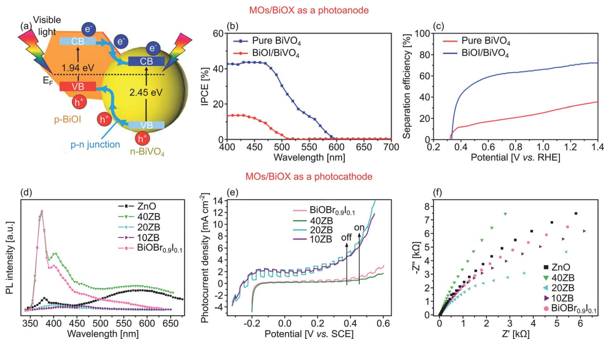
Fig. 13 (a) Photogenerated charge movement and band alignment of \text{BiVO}_4/\text{BiOI} photoanode. (b) IPCE spectra of \text{BiVO}_4 and \text{BiOI/BiVO}_4 at given wavelength at 0.68 V vs. RHE using 0.5 M \text{KH}_2\text{PO}_4 as the electrolyte. (c) Surface charge transfer efficiency using 15% \text{H}_2\text{O}_2 as a hole scavenger. (d) Photoluminescence spectra. (e) J-V curves under chopped visible light of, and (f) EIS Nyquist plot of \text{ZnO/BiOBr}_{0.9}\text{I}_{0.1} (ZB) heterostructures as a photocathode, alongside control \text{ZnO} and \text{BiOBr}_{0.9}\text{I}_{0.1} . Numbers 10, 20, and 40 denote ZnO wt%. Figures adapted with permission from: (a–c) ref. 66. Copyright 2015 Elsevier B.V. (d–f) Ref. 198. Copyright 2020 Elsevier B.V.
