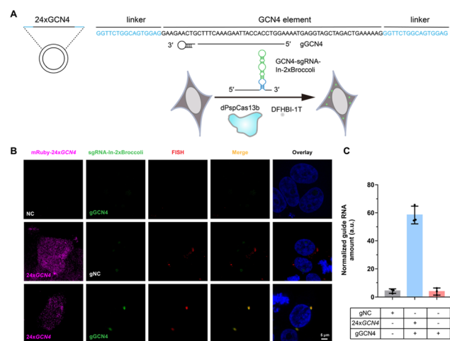
Fig. 1 Labeling GCN4 Repeats by sgRNA-In-2 \times Broccoli. (A) Schematic drawing of the GCN4 repeats labeling by CasFAS system. (B) Representative images of sgRNA-In-2 \times Broccoli labeling exogenous 24 \times GCN4 colocalized with smFISH in fixed HEK 293T cells. Upper row, negative control of exogenous 24 \times GCN4 , the cells were transfected with pGCN4-sgRNA-In-2 \times Broccoli (gGCN4: with spacer sequence targeting GCN4 ) and pdPspCas13b-2 \times NLS; middle row, the cells were transfected with pmRuby-24 \times GCN4 , psgRNA-In-2 \times Broccoli (gNC: as a negative control of spacer sequence) and pdPspCas13b-2 \times NLS; bottom row, the cells were cotransfected with pmRuby-24 \times GCN4 , pGCN4-sgRNA-In-2 \times Broccoli (gGCN4) and pdPspCas13b-2 \times NLS. The cell nucleus was dyed by Hoechst. (C) RT-qPCR analysis of GCN4 -sgRNA-In-2 \times Broccoli RNA levels in (B). All data are presented as the mean \pm s.d.; n = 3 independent experiments.
