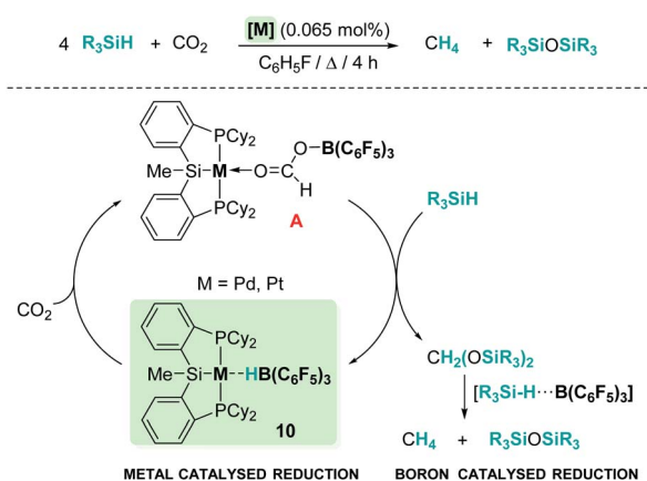
Scheme 3 Hydrosilylation of \text{CO}_2 catalysed by complexes [(\text{Cy-PSiP})\text{M}][\text{HB}(\text{C}_6\text{F}_5)_3] , 10 .
