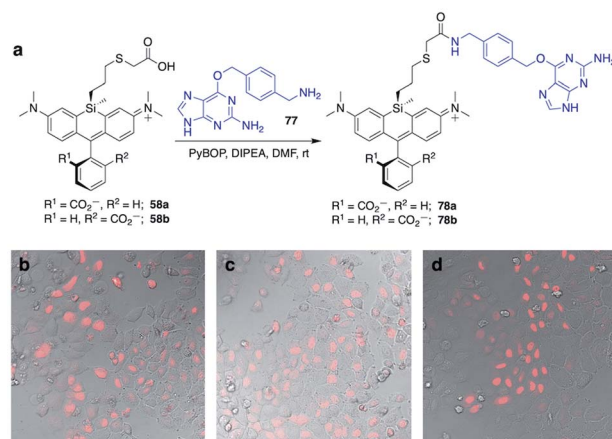
Fig. 4 Synthesis of Si-bridge dyes 78a – b and their use for live-cell imaging of HeLa cells transfected with pSNAPf-H2B. (a) Synthesis of 78a – b by the reaction of 58a – b with O 6 -benzylguanidine coupling partner 77 ; (b–d) Overlay of dye fluorescence and DIC for cells treated with 3 μM (b) SNAP-Cell 647-SiR, (c) 78a , or (d) 78b . Scale bar is 20 μm.
