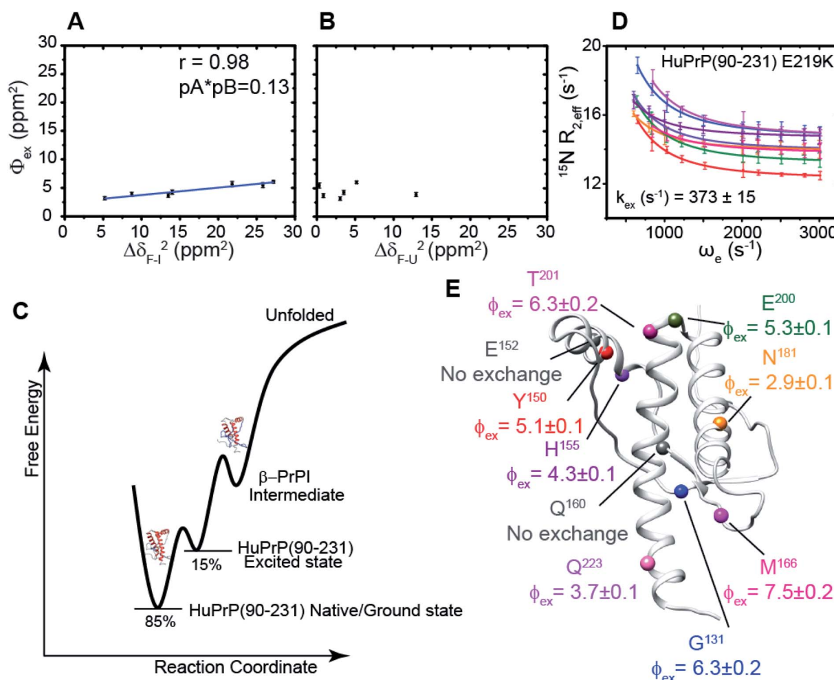
Fig. 6 Correlation between relaxation dispersion/thermal unfolding data. (A and B) \Phi_{ex} parameters ( \text{ppm}^2 ) derived from the global fit of cluster A ( k_{ex} = 2502 \pm 106 ( s^{-1} )) of HuPrP(90–231) plotted as a function of the squared differences in chemical shift between the native and the intermediate state ( \Delta\delta_{F-I} ) 2 ( \text{ppm}^2 ) (A) and between the native and the denaturated state ( \Delta\delta_{F-U} ) 2 ( \text{ppm}^2 ) (B). (C) Conformational landscape of HuPrP(90–231) revealed by NMR relaxation dispersion and thermal melt data. (D) Best fit curves to a two-site exchange model assuming a common motion for residues of HuPrP(90–231) E219K. (E) Mapping of the residue-specific \Phi_{ex} parameters extracted for HuPrP(90–231) E219K from the global fit. The residues that do not show any RD profile are reported as dark grey spheres.
