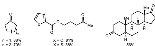
Scheme 16 Thiol radical-enabled C(sp 3 )-H elaborations.
