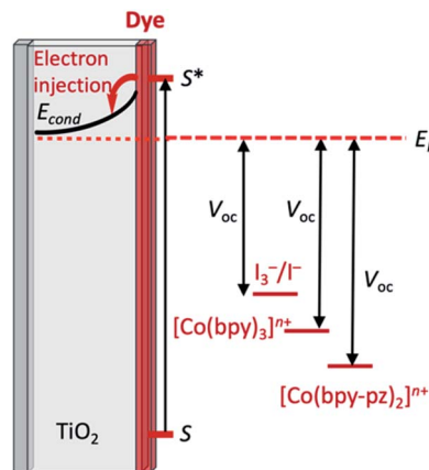
Fig. 3 Schematic illustration of the relative E_{\text{redox}} levels (in red) for two representative \text{Co}^{3+}/\text{Co}^{2+} redox mediators with respect to the \text{I}_3^-/\text{I}^- couple and the effect on the value of V_{\text{OC}} (see Fig. 2a for complete DSC diagram).
