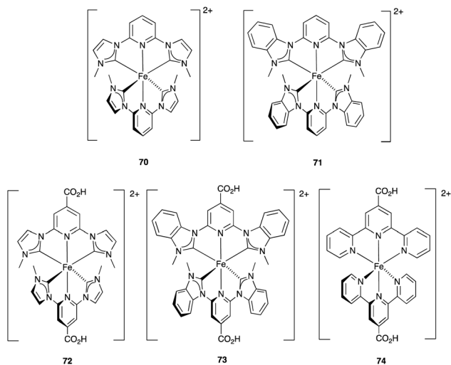
Scheme 25 Structures of the homoleptic NHC iron(II) complexes 70–73 and of [\text{Fe}(\text{4'–HO}_2\text{Ctpy})_2]^{2+} (74).
