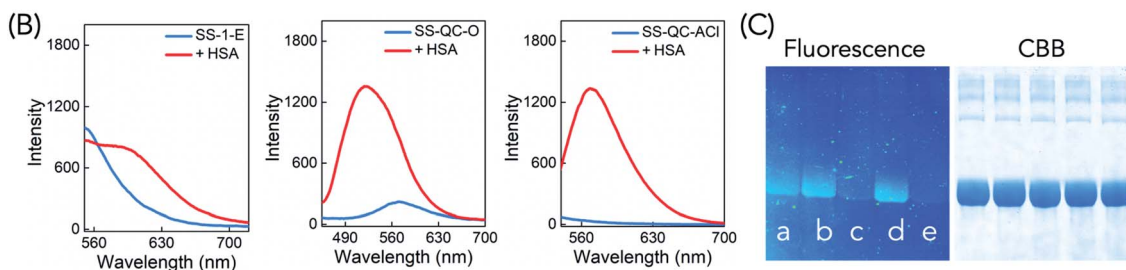
Fig. 2 Covalent binding site verification of HSA and SS-1. (A) Reaction site based modification of the fluorescent dyes. (B) Fluorescence responses of 5 \mu\text{M} SS-1-E, SS-QC-O and SS-QC-ACI toward HSA (2 \text{mg mL}^{-1} for SS-1-E, 0.5 \text{mg mL}^{-1} for SS-QC-O and SS-QC-ACI) in PBS, respectively. SS-1-E: \lambda_{\text{ex}} = 516 , slit 5/5 nm, 700 V; SS-QC-O: \lambda_{\text{ex}} = 440 , slit 2.5/5 nm, 700 V; SS-QC-ACI: \lambda_{\text{ex}} = 505 , slit 2.5/5 nm, 700 V. (C) Covalent labeling verification of HSA by SS-1, SS-1-E, SS-QC-O or SS-QC-ACI analyzed by SDS-PAGE gel. (a–d) Represent the addition of the four fluorescent dyes (40 \mu\text{M} ) to HSA (1.25 \text{mg mL}^{-1} ), respectively; (e) is the control group without dye addition.
