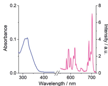
Fig. 2 Absorption (blue) and emission (pink) spectrum of [\text{Eu} \cdot \text{mBOH}_2]^+ ( 5 \mu\text{M} ) in 10 mM HEPES at pH 7.0 and 295 K, \lambda_{\text{exc}} = 322 \text{ nm} .
