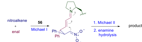
Scheme 40 Formal [2 + 2] cycloaddition of nitroalkenes to enals catalyzed by bifunctional squaramide 56 .
