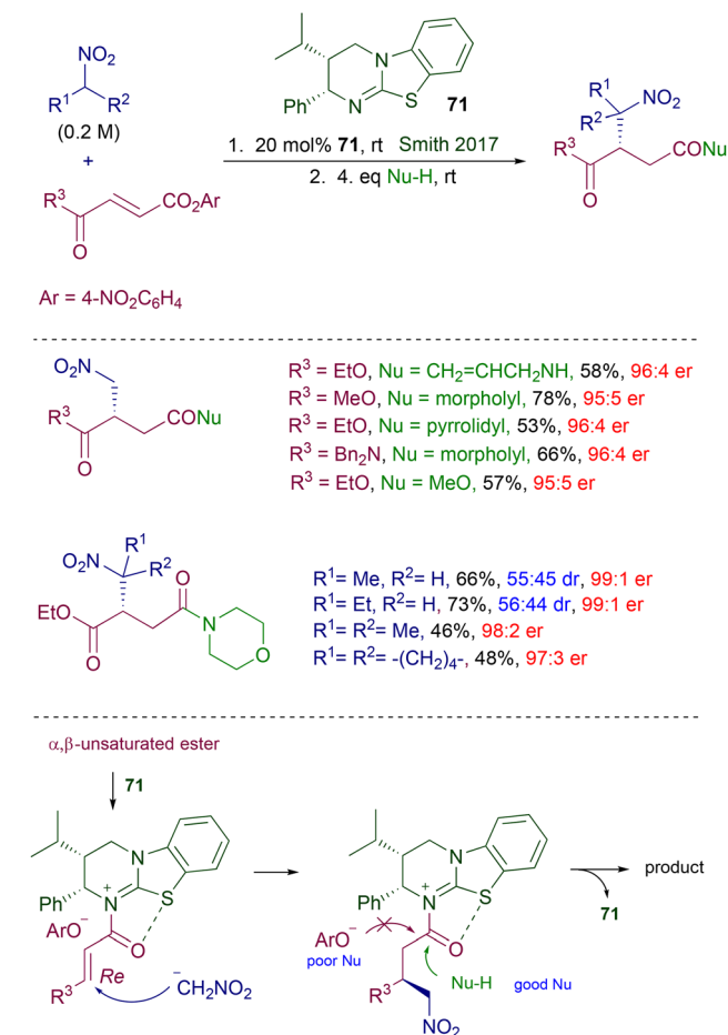
Scheme 53 Enantioselective conjugate addition of nitroalkanes to fumaric acid derivatives via chiral acylammonium ion intermediate.
