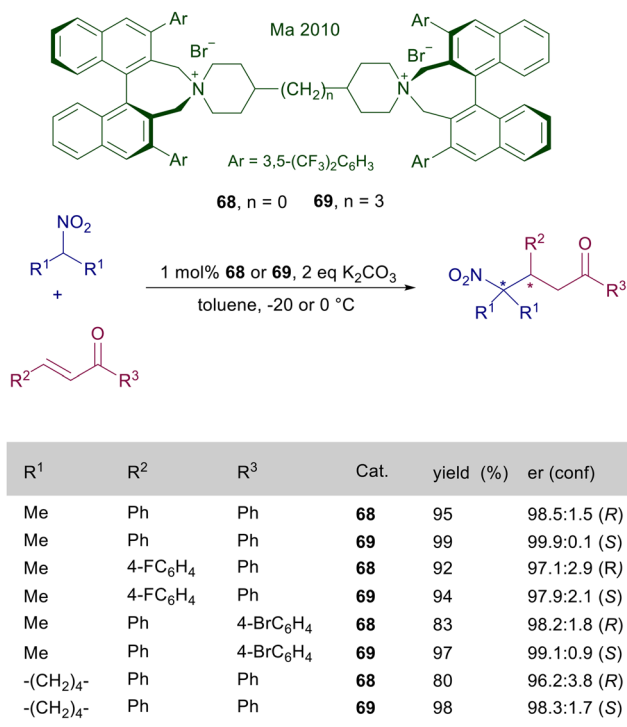
Scheme 51 Enantiodivergent conjugate addition of tertiary nitroalkanes to chalcones catalyzed by differently tethered ammonium salts 68 and 69 .
