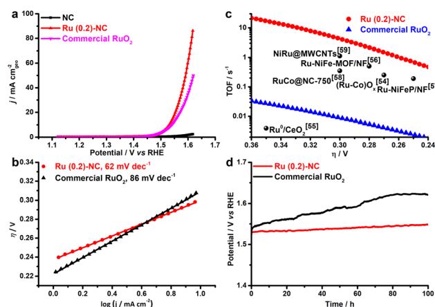
Fig. 3 Electrocatalytic OER performance of Ru (0.2)-NC and other control catalysts. (a) LSV curves. Scan rate: 5 \text{mV s}^{-1} . (b) Tafel slopes. (c) Comparison of the TOF values with other state-of-the-art OER catalysts. (d) Long-term catalytic stability test at 10 \text{mA cm}^{-2} in 1.0 M KOH.
