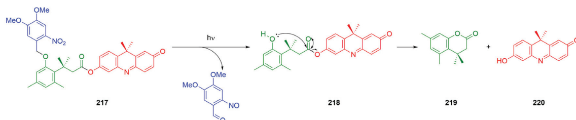
Scheme 49 Near-UV triggered self-immolative system 217 cable of undergoing a trimethyl-lock accelerated cyclisation event resulting in the release of a fluorescent reporter moiety as described by Jullien, Schmidt and co-workers. 199
