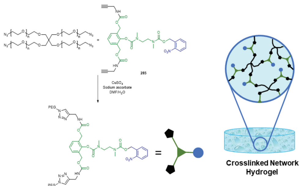
Scheme 62 The light-triggered self-immolative hydrogel reported by Gillies and co-workers. 260
