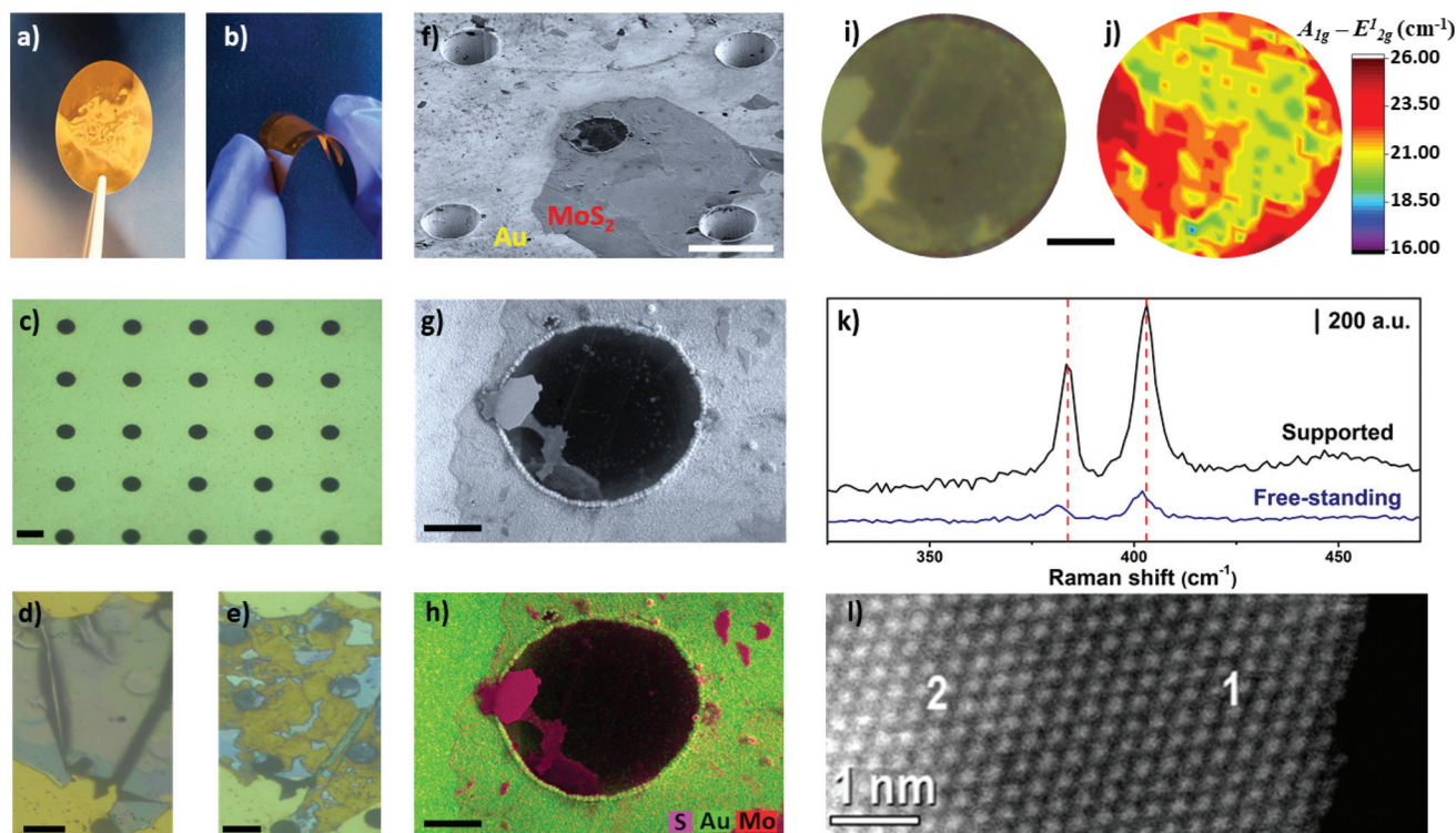
Fig. 6 (a and b) Photos of the microhole-structured Ni/Au mesh. (c) Optical microscopy image of the Au mesh. Scale bar is 20 \mu m. (d and e) Optical microscopy images of the MoS 2 flakes before and after electrochemical thinning process, respectively. Scale bar is 25 \mu m. (f) Tilted secondary electron SEM image of the thinned flake on the Au micromesh. Scale bar is 25 \mu m. (g and h) High-magnification secondary electron SEM image of thinned area on the microhole and EDS map, respectively. Scale bar is 5 \mu m. (i and j) Optical microscope image of the microhole region and Raman map, respectively. Scale bar is 5 \mu m. (k) Raman spectra obtained on supported and free-standing areas as indicated. (l) HAADF-HRSTEM image of the electrochemically thinned MoS 2 layer. The inset numbers 1 and 2 indicated mono and bilayer regions, respectively.
