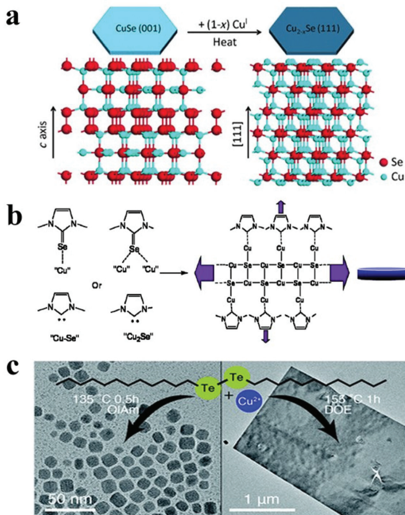
Fig. 5 (a) Schematic illustrating transformation from hexagonal CuSe to cubic \text{Cu}_{2-x}\text{Se} under heat treatment due to insertion of \text{CuI} ; reproduced from ref. 122 with permission from Wiley, copyright 2014; (b) mechanism of cubic \text{Cu}_{2-x}\text{Se} nanodisc formation via imidazoline-2-selenone interaction with NC surface; reproduced from ref. 125 with permission from ACS, copyright 2010; (c) formation of \text{Cu}_{2-x}\text{Te} NCs and vulcanite nanosheets under different reaction condition using di-dodecyl ditelluride as the Te precursor. Reproduced from ref. 127 with permission from RSC, copyright 2020.
