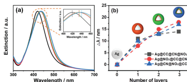
Fig. 3 (a) Normalized UV-vis spectra of Ag NPs (black line), Ag@CN (red line), Ag@CN@NO 2 (green line) and Ag@CN@NO 2 @CCH (blue line); (b) Plot of \Delta\lambda (red shift of plasmon band) vs. the number of grafted layers around Ag cores for the step-by-step functionalization of Ag@CCH@CN@NO 2 , Ag@NO 2 @CCH@CN and Ag@CN@NO 2 @CCH.
