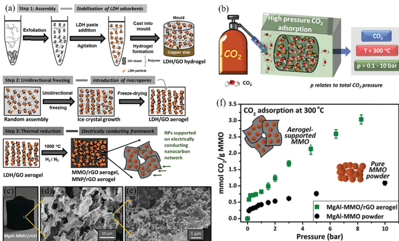
Fig. 8 Adsorption of \text{CO}_2 with MMO/RGO hybrid aerogel: (a) Synthesis process. (b) MgAl-MMO/RGO aerogel high pressure precombustion \text{CO}_2 adsorption schematic diagram. (c) Photograph of MgAl-MMO/RGO aerogel. (d and e) SEM images of MgAl-MMO/RGO aerogels. (f) The high-pressure \text{CO}_2 adsorption isotherm on MgAl-MMO powder and MgAlMMO/RGO aerogel under the condition of 300 °C and \text{CO}_2 total pressure of 0.210 bar. 149 Copyright 2020, Wiley-VCH.
