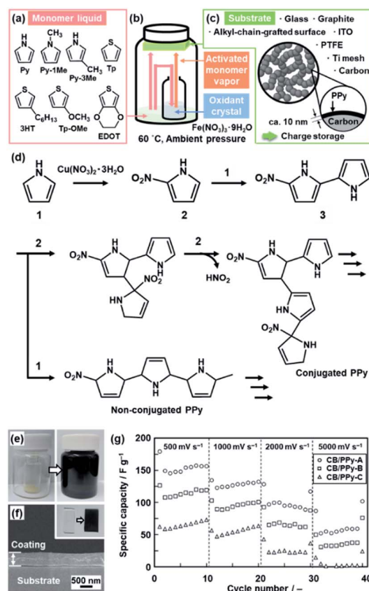
Fig. 4 Polymerization of the heteroaromatic monomer and its activation on substrates. (a) Molecular structures of the heteroaromatic monomers, such as the pyrrole (Py) and thiophene (Tp) derivatives. (b) Experimental setup for the coating. (c) Substrates for the coating and its application to the energy storage. (d) Synthetic routes of the conjugated and nonconjugated PPy from Py and nitrated Py generated on the surface of the Cu(NO 3 ) 2 ·3H 2 O crystals. (e) Photographs of the sample bottle before (left) and after (right) the coating of PPy. (f) Photograph (the inset) and the cross-sectional SEM image of the PPy coating on a glass substrate for 1 h. (g) Relationship between the scan rate and specific capacity of the samples with the coating time 1 h for CB/PPy-A, 3 h for CB/PPy-B, and 6 h for CB/PPy-C. Reproduced from ref. 22a and b with permission from the Royal Society of Chemistry.
