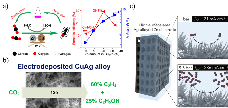
Fig. 10 (a) Schematic diagram of ethanol production from \text{CuZn} alloy. Reproduced with permission. 58 Copyright 2016, American Chemical Society. (b) Schematic diagram of the production of \text{C}_2 products from \text{CuAg} alloys. Reproduced with permission. 17 Copyright 2018, American Chemical Society. (c) Schematic diagram of efficient CO production from \text{AgZn} alloy. Reproduced with permission. 27 Copyright 2019, Elsevier Inc.
