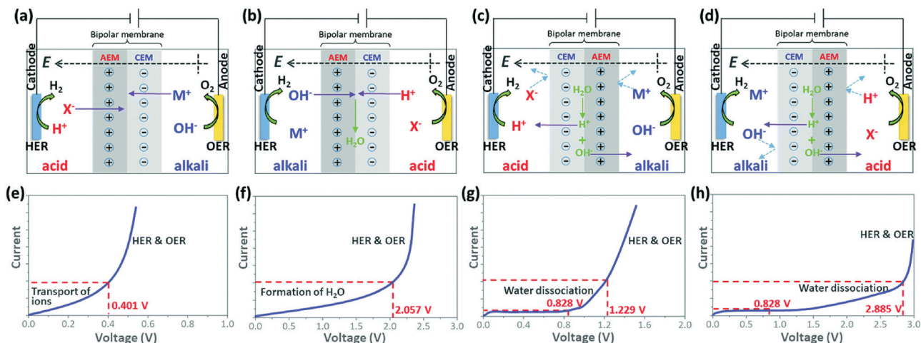
Fig. 18 (a–d) Schematic illustrations of four water electrolyser configurations using acid–base asymmetric electrolytes in two compartments separated by a BPM: (a) acidic cathode|AEM|CEM|alkaline anode, (b) alkaline cathode|AEM|CEM|acidic anode, (c) acidic cathode|CEM|AEM|alkaline anode, and (d) alkaline cathode|CEM|AEM|acidic anode. (e–h) Theoretical I – V curves of the four configurations corresponding to (a–d). Reproduced from ref. 316 with permission from the Royal Society of Chemistry.
