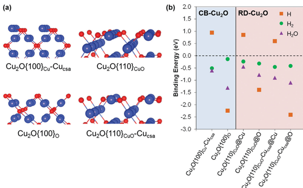
Fig. 3 (a) Atomic arrangement of thermodynamically stable Cu 2 O {100} and {110} exposed facet with distinctive terminating surface, blue represents Cu atom and red represents O atom, and (b) modelled surface adsorption ability of H, H 2 and H 2 O of Cu 2 O {100} and {110}. Cu 2 O{100} Cu -Cu csa : Cu-terminated Cu 2 O{100} with a coordinatively saturated Cu removed, Cu 2 O{100} O : O-terminated Cu 2 O{100}, Cu 2 O{110} CuO : CuO-terminated Cu 2 O{110} and Cu 2 O{110} CuO -Cu csa : CuO-terminated Cu 2 O{110} with coordinatively saturated Cu removed. The @O and @Cu denotes adsorption at O and Cu active sites, respectively.
