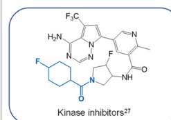
Fig. 1 Synthetic strategies for the production of fluorinated cycloalkane derivatives, and examples of applications.
