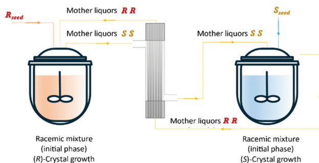
Fig. 14 Schematic representation of the hybrid crystallization/filtration process. By seeding the vessels, it will promote the preferential crystallization of a specific enantiomer. The counter enantiomer rich mother liquors will flow through the membrane only transporting the dissolved compounds.
