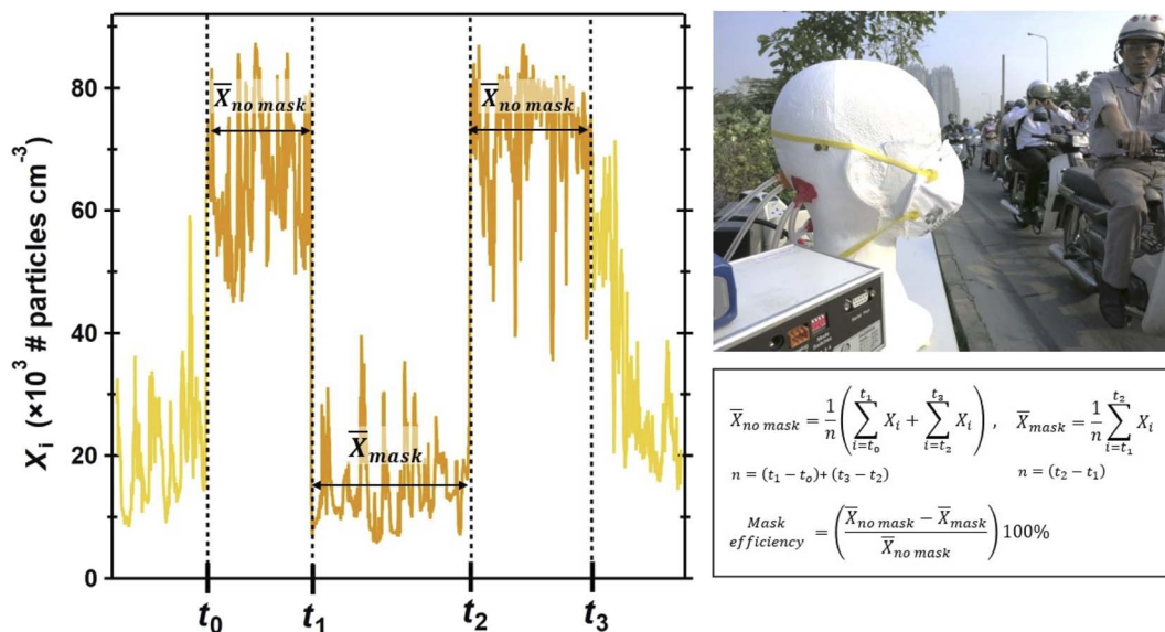
Fig. 3 Mask efficiency tests. The particle instruments were connected by sampling tubes passing from the back to the front (nose area) of the manikin. Each test consisted of three \sim 10 min sampling periods. The particle concentration without a mask ( \bar{X}_{no\ mask} ) was obtained in the first and third periods, and the concentration with a mask ( \bar{X}_{mask} ) during the second period. The total inward leakages of the masks were calculated based on the formulae outlined.
