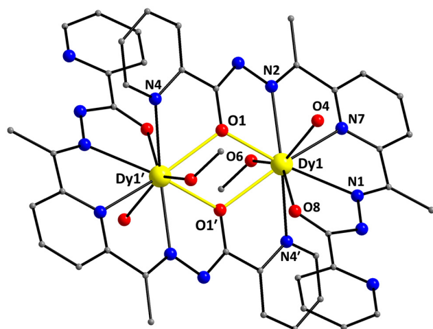
Fig. 3 Partially labelled representation of the [\text{Dy}_2(\text{LH})_2(\text{MeOH})_2(\text{H}_2\text{O})_2]^{4+} cation that is present in the crystal of 3 ·2MeOH, highlighting the \{\text{Dy}_2(\mu\text{-OR})_2\}^{4+} core with yellow thick bonds. H atoms are omitted for clarity. Color scheme as in Fig. 1. Symmetry code: (') 1 - x, 1 - y, 1 - z .
