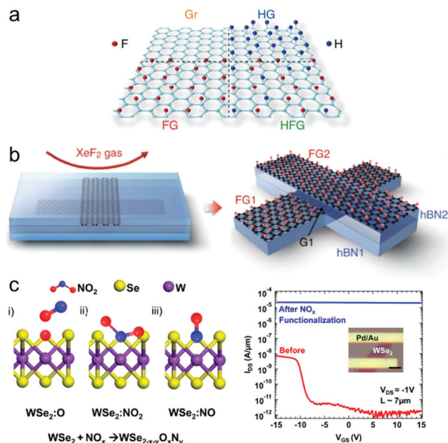
Fig. 9 (a) Patterned graphene surface functionalization by plasma hydrogenation and fluorination by \text{XeF}_2 (reprinted with permission from ref. 199 Copyright 2019 Advanced Materials). (b) Etching and functionalization process of graphene/hBN heterostructure by \text{XeF}_2 . hBN layers are etched away while graphene is fluorinated (reprinted with permission from ref. 217 Copyright 2018 nature communications). (c) Three possible reaction configurations between Se vacancy of \text{WSe}_2 and \text{NO}_2 gas (left) and transfer curve before/after \text{NO}_2 treatment (right) (reprinted with permission from ref. 135 Copyright 2014 ACS Nano).
