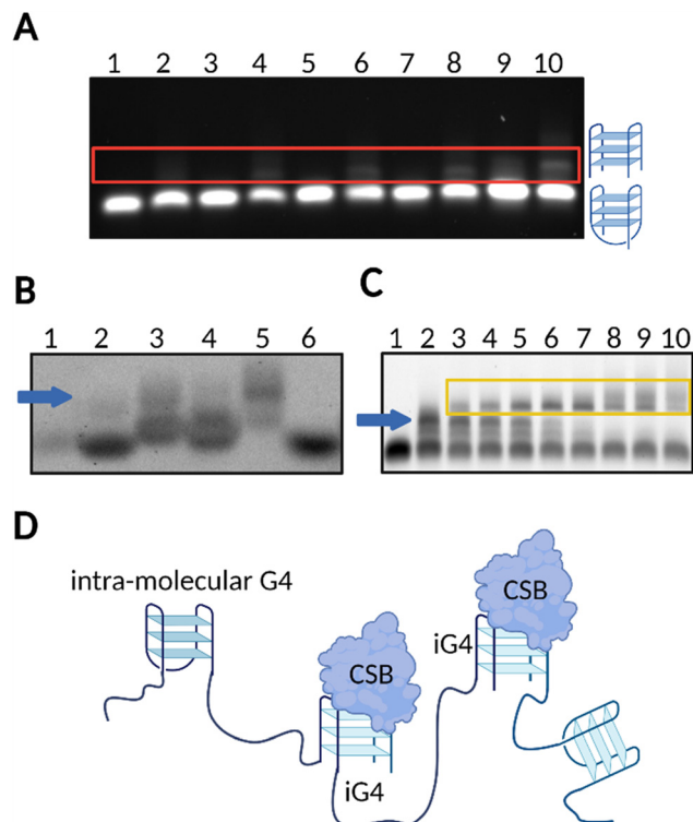
Fig. 2 rDNA sequences form iG4s that are selectively bound by CSB. (A) Native gel electrophoresis showing that untailied rDNA is not able to form iG4s in the presence of \text{Li}^+ or \text{K}^+ (lanes 1 and 2, respectively). A tail of at least 3–5 bp is required for iG4s to form under \text{K}^+ conditions (upper bands displayed in lanes 4 and 6, respectively), but not under \text{Li}^+ conditions (lanes 3 and 5). A longer tail of 10–20 bp allows the formation of more stable iG4s which can mostly form in presence of \text{K}^+ (lanes 8 and 10, respectively) compared to \text{Li}^+ conditions (lanes 7 and 9). (B) NMM staining of agarose gel confirmed formation of folded G4 structures from rDNA sequences (lane 2: untailied rDNA in \text{K}^+ ; lane 3 to 5: tailied rDNAs under \text{K}^+ conditions; lane 6: untailied rDNA in \text{Li}^+ ). ssDNA remained unstained (lane 1). iG4 bands are indicated with a blue arrow. (C) Agarose EMSA gel on tailied rDNA G4 using increasing concentrations of CSB in \text{K}^+ conditions (lanes 2–10). Lane 1 is a control with the oligonucleotide annealed in \text{Li}^+ . iG4 bands are indicated with a blue arrow while the interaction between the iG4 and CSB is indicated within a yellow box. (D) Schematic representation of the selective binding of CSB towards iG4s. 13
