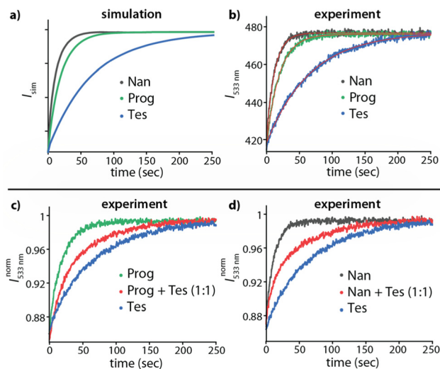
Fig. 4 (a) Simulated kinADA and (b) Experimental kinADA PFO traces monitored at 533 nm ( \lambda_{\text{exc}} = 376 nm) for CB8 \rightarrow Tes (1 \mu M, blue), CB8 \rightarrow Prog (1 \mu M, green) and CB8 \rightarrow Nan (1 \mu M, black) host \rightarrow analyte complex upon spiked addition of MPCP dye (50 \mu M) in water. See Fig. S5 and S6 in the ESI† for further details and parameters used for the simulation. The red line in Fig. 4b depicts the fitted data according to the kinADA PFO binding model (eqn (1)). Experimental kinADA PFO traces monitored at 533 nm ( \lambda_{\text{exc}} = 376 nm) for a mixture of two steroids as analytes (red curve) in case of (c) CB8 (1 \mu M), Tes (0.5 \mu M) and Prog (0.5 \mu M) and (d) CB8 (1 \mu M), Tes (0.5 \mu M) and Nan (0.5 \mu M) upon spiked addition of MPCP (50 \mu M) in water. The kinetic traces for individual steroids are shown for comparison.
