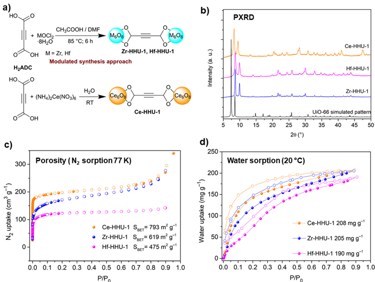
Fig. 34 (a) Reaction schemes for the synthesis of M-HHU-1 ( \text{M} = \text{Zr}, \text{Hf}, \text{Ce} ), (b) powder X-ray diffraction patterns of M-HHU-1 ( \text{M} = \text{Zr}, \text{Hf}, \text{Ce} ), compared with the simulated pattern for UiO-66, (c) nitrogen adsorption isotherms at 77 K, and (d) water sorption isotherms of M-HHU-1 ( \text{M} = \text{Zr}, \text{Hf}, \text{Ce} ) at 20^\circ\text{C} . Graphics adapted from ref. 34, 90 and 94.
