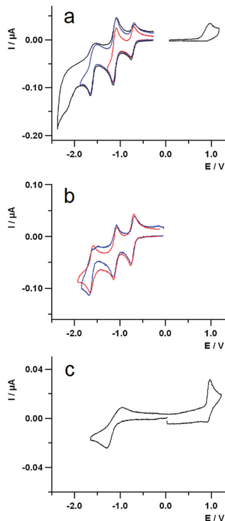
Fig. 4 Cyclic voltammetric curves of (a) 0.6 mM species 3 (three scans at different inversion potential); (b) 0.7 mM compound C 60 -Ph (blue line) and 5 (red line); (c) 0.7 mM species 4 recorded in TBAH/DCM at 298 K. Scan rate = 1 V s −1 ; working electrode: platinum disk (diameter 125 μm); reference electrode: SCE.
