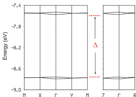
Fig. 11 Calculated three-dimensional band structure for the donor sublattice of [(rac)-\mathbf{1}]_2(\text{Mo}_6\text{O}_{19}) , where \Gamma = (0, 0, 0) , X = (a^*/2, 0, 0) , Y = (0, b^*/2, 0) , M = (a^*/2, b^*/2, 0) , Z = (0, 0, c^*/2) and R = (a^*/2, b^*/2, c^*/2) . \Delta is the energy gap between the filled and empty bands.
