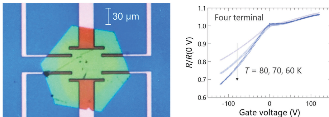
Fig. 9 Microscope image of the thin hexagonal crystal of [(S)-\mathbf{1}]_9(\text{Mo}_6\text{O}_{19})_5(\text{CHBr}_3)_2 attached on the \text{SiO}_2/\text{Si} substrate with pre-patterned gold electrodes (left). Gate voltage dependence of normalized resistance of the crystal at selected temperatures of 60 K, 70 K, and 80 K (right).
