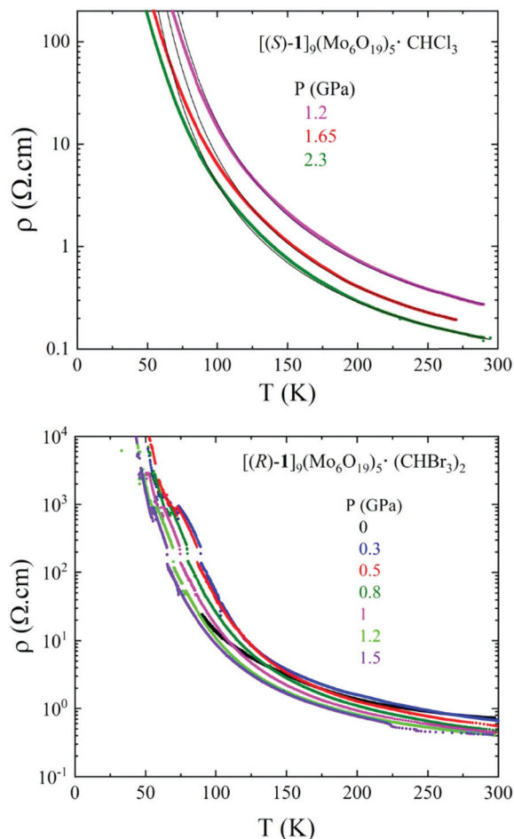
Fig. 5 Temperature dependence of the electrical resistivity \rho at different applied pressures for a single crystal of [(S)-1]_9(Mo_6O_{19})_5 \cdot CHCl_3 (top) and for a single crystal of [(R)-1]_9(Mo_6O_{19})_5 \cdot (CHBr_3)_2 (bottom).
