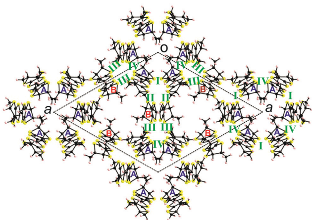
Fig. 6 Donor layer of the [(S)-1]_9(Mo_6O_{19})_5 \cdot CHCl_3 salt where the different donors and intermolecular interactions are labeled.
