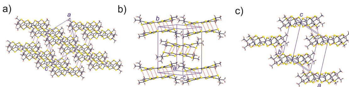
Fig. 10 Donor sublattice of the [(rac)-\mathbf{1}]_2(\text{Mo}_6\text{O}_{19}) salt. The \text{S}\cdots\text{S} contacts shorter than 3.9 Å are shown as dashed red (intra-dimer) and purple (inter-dimer) lines.
