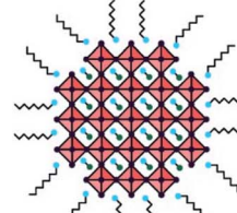
Nanocrystal (0D)
