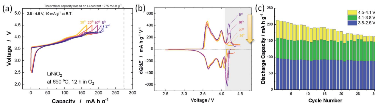
Fig. 1 (a) Galvanostatic charge/discharge curves of \text{LiNiO}_2 at a rate of 10\text{ mA g}^{-1} , (b) differential \text{d}Q/\text{d}E plots obtained from (a), and (c) variations in discharge capacities with different voltage ranges.
