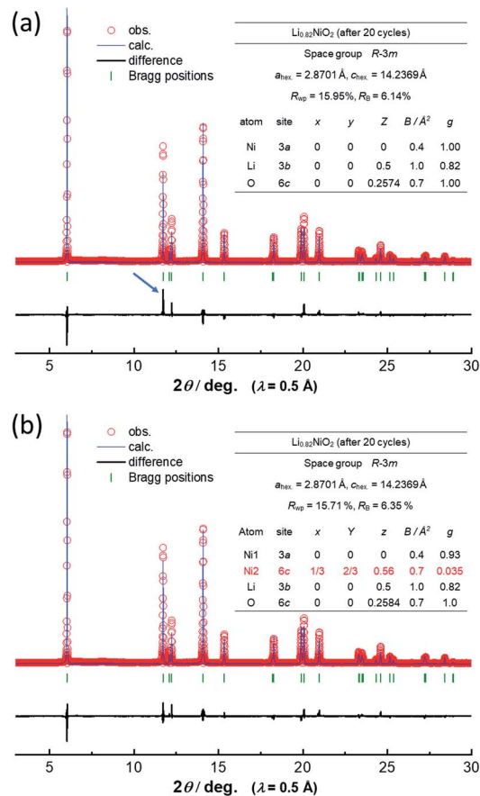
Fig. 4 Comparison of fitting results of Rietveld analysis of the synchrotron XRD pattern of Li 0.82 NiO 2 after the 20-cycle test (a) without and (b) with the presence of Ni ions at 6c tetrahedral sites. A clear deviation between simulated and observed patterns for the 10 \bar{1} diffraction line is noted in (a) as marked by the blue arrow.
