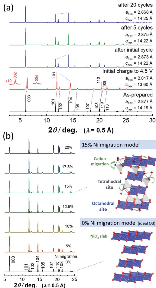
Fig. 3 (a) Synchrotron XRD patterns of \text{LiNiO}_2 before and after electrochemical cycles, and (b) simulated XRD patterns with different occupancy of Ni ions at tetrahedral 6c sites. Schematic illustrations of structural models of \text{NiO}_2 are shown, which were drawn using the program VESTA. 20
