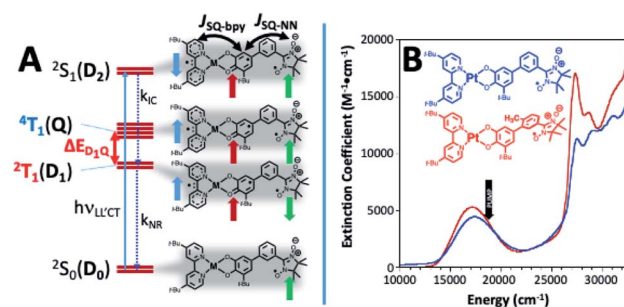
Fig. 2 (A) (Left) ground doublet- ( ^2S_0/D_0 ) and LLCT excited state manifold. Vertical doublet ^2S_1(D_2) undergoes rapid internal conversion ( k_{IC} ) to ^2T_1(D_1) , which has (bpy)Pt(CAT) triplet character. Nonradiative decay of the ^2T_1 state ( k_{NR} ) provides the ^2S_0 ground state with non-Boltzmann m_s populations. (Right) depictions of ground- ( ^2S_0/D_0 ), and LLCT excited states; magnetic exchange coupling parameters, J_{SQ-bpy} and J_{SQ-NN} defined; J_{SQ-NN} is related to J_{CR} in Fig. 1. (B) Electronic absorption spectra (300 K; CH_2Cl_2 ), for mPh-Pt (blue line) and 6-Me-mPh-Pt (red line), indicating TREPR photoexcitation energy relative to the \sim 17\,000\text{ cm}^{-1} ^2S_0(D_0) \rightarrow ^2S_1(D_2) LLCT transition
