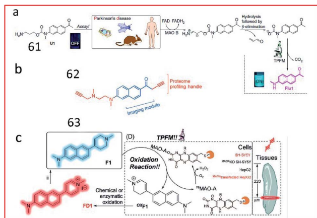
Fig. 41 Overview of the design and synthesis of MAO-specific probes. (a) 61. Reprinted from ref. 161 with permission. Copyright 2014 Macmillan Publishers Limited. (b) 62. Reprinted from ref. 162 with permission. Copyright 2015 Wiley-VCH Verlag GmbH & Co. KGaA, Weinheim. (c) 63. Reprinted from ref. 163 with permission. Copyright 2020 Wiley-VCH Verlag GmbH & Co. KGaA, Weinheim.
