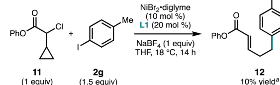
Fig. 5 Mechanistic experiments. a Determined by 1 H NMR.
