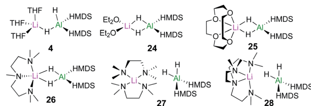
Fig. 6 Structures of lithium aluminates [(\text{D})_x\text{LiAlH}_2(\text{HMDS})_2] ( 4 , 24–28 ) ( x = 2 for \text{THF} , \text{OEt}_2 , \text{TMEDA} ; x = 1 for 12\text{-c-4} , \text{PMDETA} and \text{Me}_6\text{-Tren} ).
