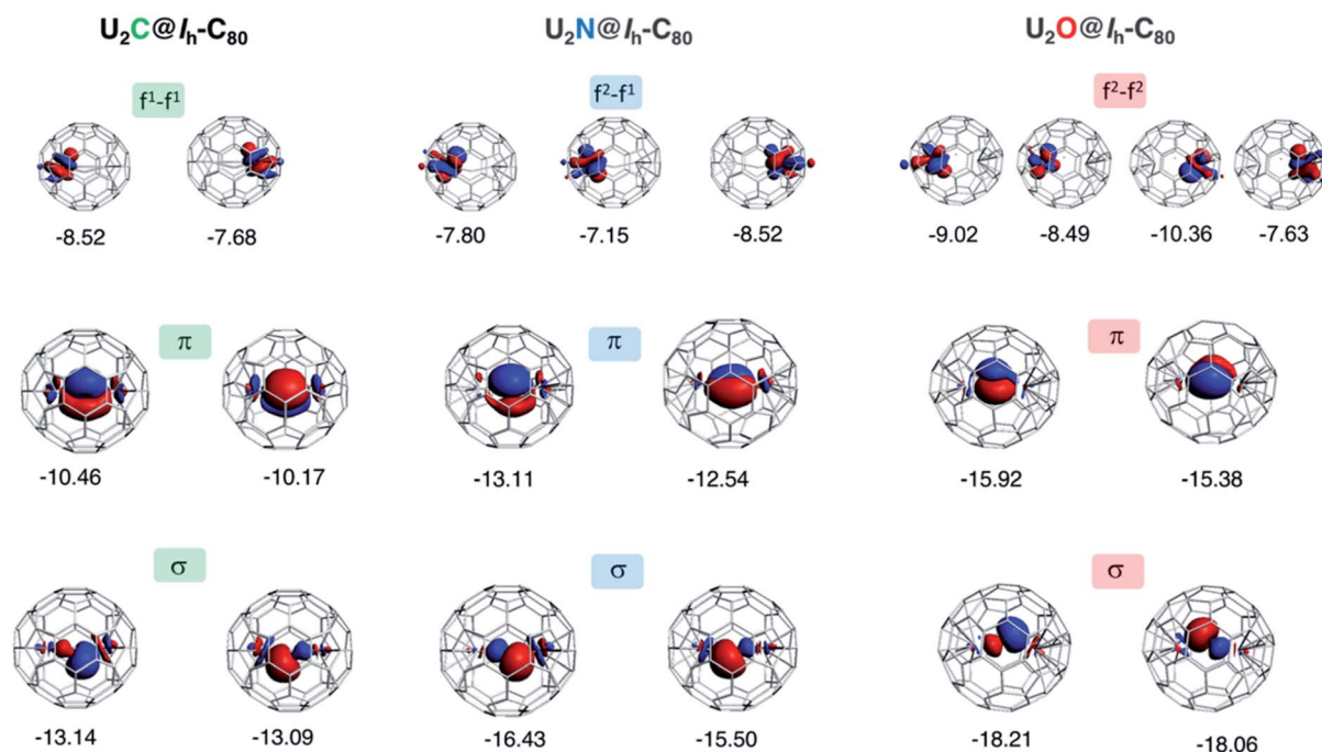
Fig. 6 Localized (Boys–Foster) MOs for \text{U}_2\text{X}@\text{C}_{80} with \text{X} = \text{C}, \text{N} and \text{O} . MOs relevant to bonding in the \text{U}_2\text{X} moiety are represented. The orbital energies (in eV) of non-bonding f electrons of U do not depend significantly on X, but \pi and \sigma orbitals are much more sensitive to the central atom. The modest multiple bond nature of \text{U}=\text{X} interaction decreases further as electronegativity of X increases. Orbital compositions are given in Table S2.†
