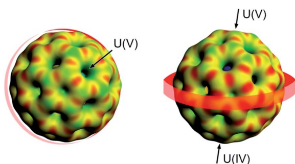
Fig. 5 Two views of the molecular electrostatic potential (MEP) for \text{U}_2\text{N}@\text{C}_{80} . Red identifies regions in which the MEP is low (nucleophilic regions) and green identifies regions where the MEP is high (electrophilic regions). The equatorial region between the two U atoms, found to be the most electrophilic part of the cage, is highlighted with a red belt.
