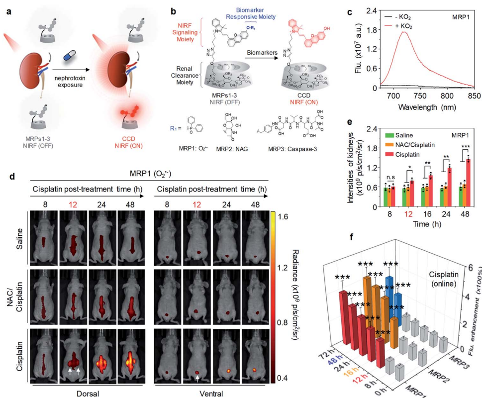
Fig. 5 (a) Schematic illustration of NIRF imaging of drug-induced AKI using MRPs1–3. (b) Chemical structures and molecular mechanisms of MRPs1–3 and their activated forms in response to \text{O}_2^{\cdot-} , NAG and caspase-3, respectively ( R = \text{H} or \text{CH}_2\text{CHOHCH}_3 ). (c) Fluorescence spectra of MRP1 (30 \mu\text{M} ) in the absence or presence of \text{KO}_2 (60 \mu\text{M} ) in PBS buffer (10 mM, pH 7.4). (d) Representative NIR fluorescence images of living mice with injection of MRP1 after treatment of cisplatin (20 mg per kg body weight) for 8, 12, 24 or 48 h. The control groups were treated with PBS or a nephroprotective antioxidant NAC. NIRF images acquired at 720 nm upon excitation at 675 nm. (e) NIRF intensities of kidneys in living mice after 30 min injection of MRP1 at the different post-treatment time points (8, 12, 16, 24 or 48 h). (f) Fluorescence enhancement of excreted MRPs1–3 in the urine from cisplatin-treated living mice after injection at different time points post-treatment of cisplatin. n.s.: not significant, *p < 0.05 , **p < 0.01 , ***p < 0.001 . Reproduced with permission from ref. 56. Copyright 2019 Springer Nature.
