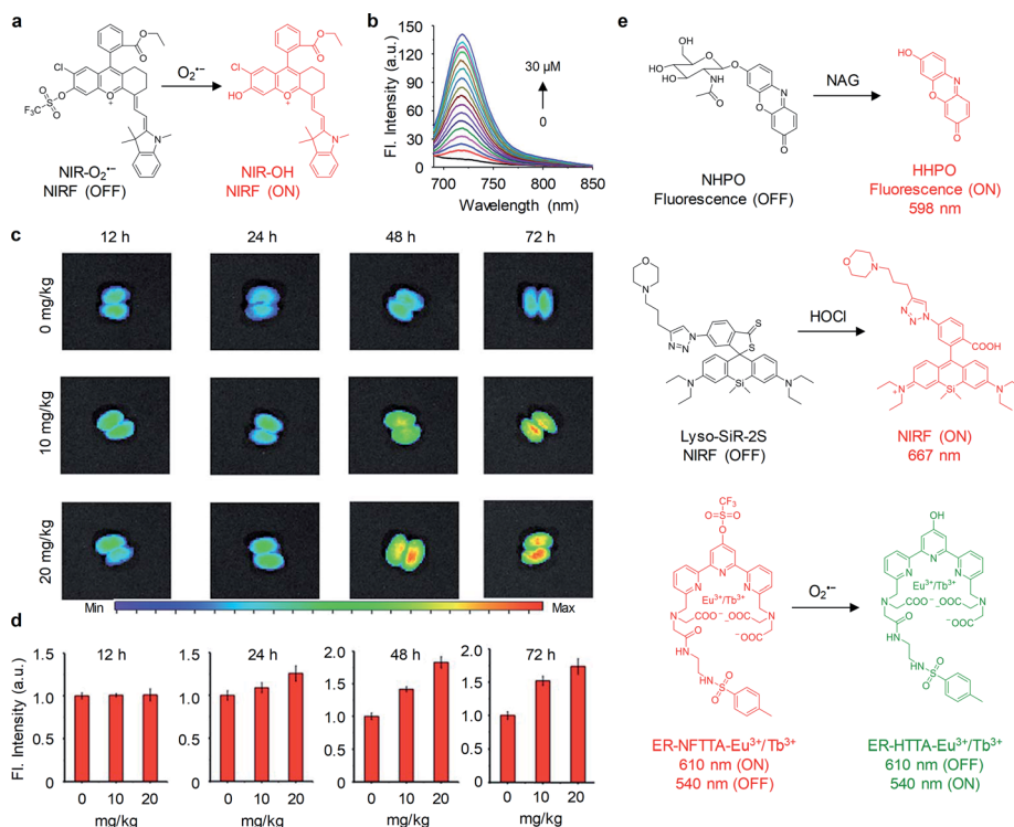
Fig. 7 (a) Chemical structures of \text{NIR-O}_2^- and its activation form in response to \text{O}_2^- . (b) Fluorescence spectra of \text{NIR-O}_2^- ( 5 \mu\text{M} ) in PBS ( 25 \text{ mM} , \text{pH } 7.4 ) upon addition of \text{O}_2^- ( 0 – 30 \mu\text{M} ). (c) Representative NIFR images of excised kidneys from mice treated with different doses of cisplatin ( 0 , 10 and 20 \text{ mg kg}^{-1} ) at different post-treatment time points ( 12 , 24 , 48 and 72 \text{ h} ). (d) NIFR intensities of the kidneys in panel c. (e) Chemical structures of probes NHPO , Lyso-SiR-2S and ER-NFTTA-Eu 3+ /Tb 3+ and their activation forms in response to NAG , HClO and \text{O}_2^- , respectively. Reproduced with permission from ref. 59. Copyright 2018 Royal Society of Chemistry.
