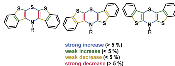
Fig. 3 Relative change of Wiberg bond orders \Delta(\text{BO}_{x+}-\text{BO}_x) from neutral precursors 5, 6, and 7 to radical cations 5 + , 6 + , and 7 + in the BBTT core (R = p -fluorophenyl; uB3LYP/6-311G**) (A detailed list of bond orders is given in the ESI†).
