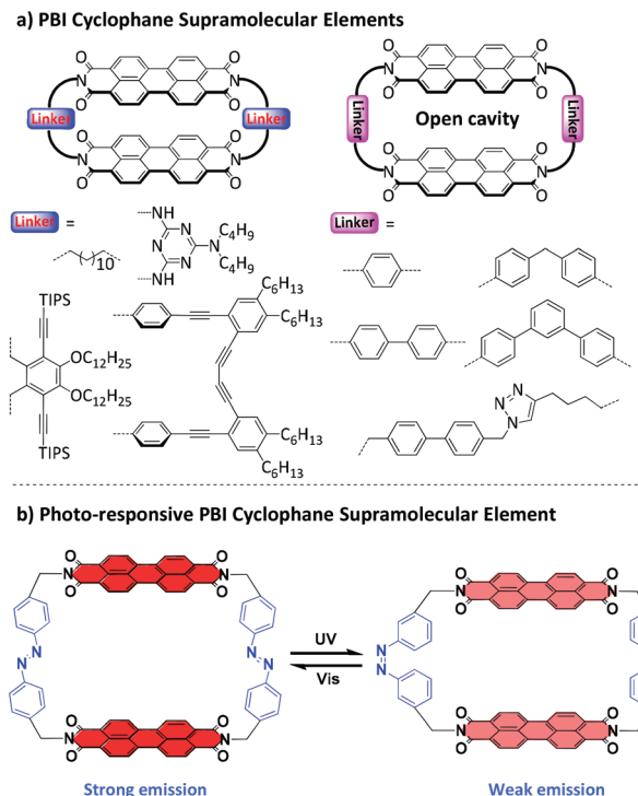
Fig. 1 Schematic illustration of PBI cyclophane supramolecular elements. (a) Representative PBI cyclophane supramolecular elements with rigid linkers. (b) PBI cyclophane supramolecular element with photoresponsive linkers, which showed reversible structural and fluorescence switching under alternate UV and visible light irradiation. Notes: The bay-position substituents of the PBIs are omitted for clarity. For details of the PBI cyclophane structures illustrated in (a), the original literature reports 21–25 should be consulted.
